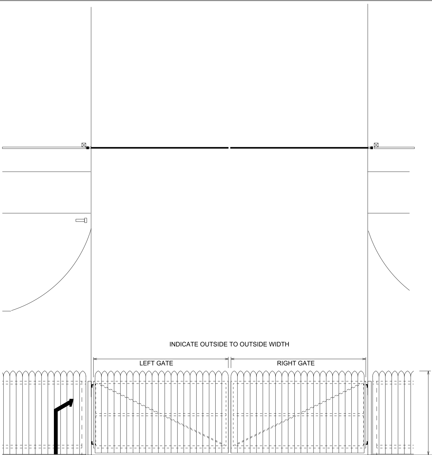
HIGH DOUBLE WOOD / VINYL GATE ( 8'-0" OR MORE WIDE ) EXTERIOR ELEVATION
